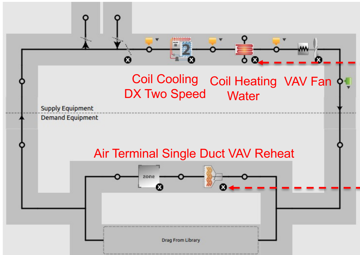
Air loop
