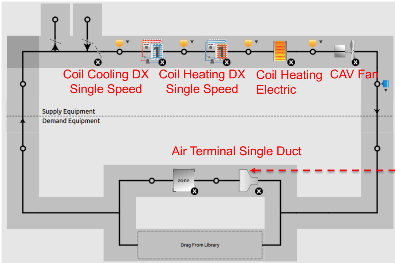
Air Loop
