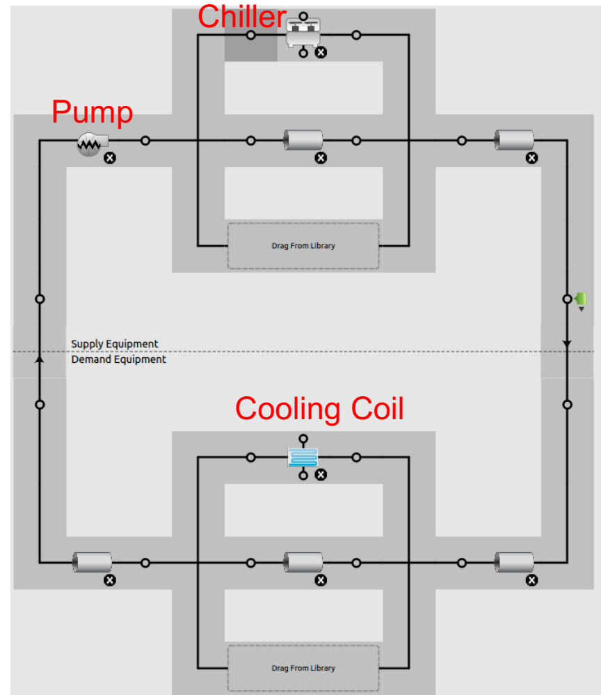
Chilled water Loop
