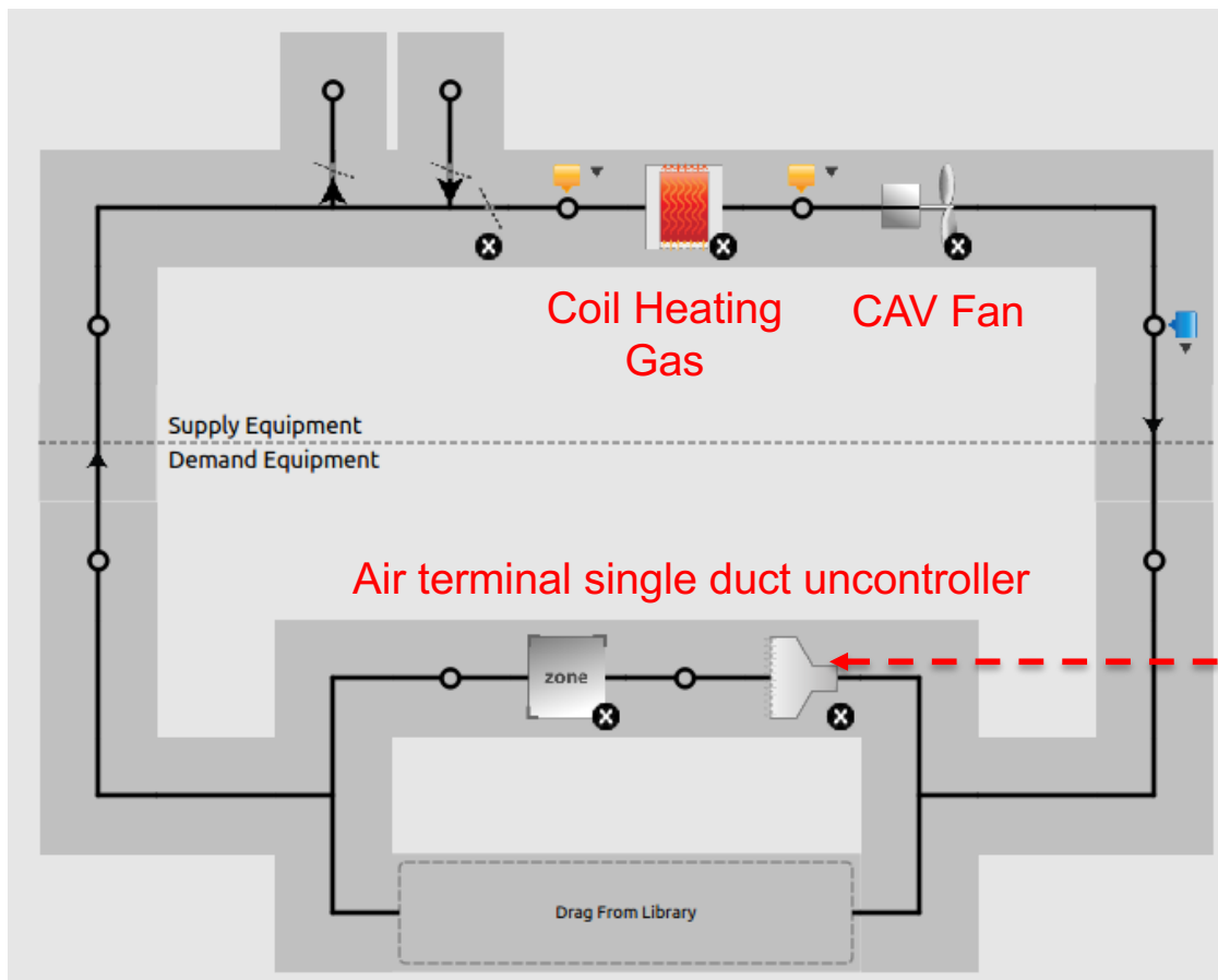
Air Loop
