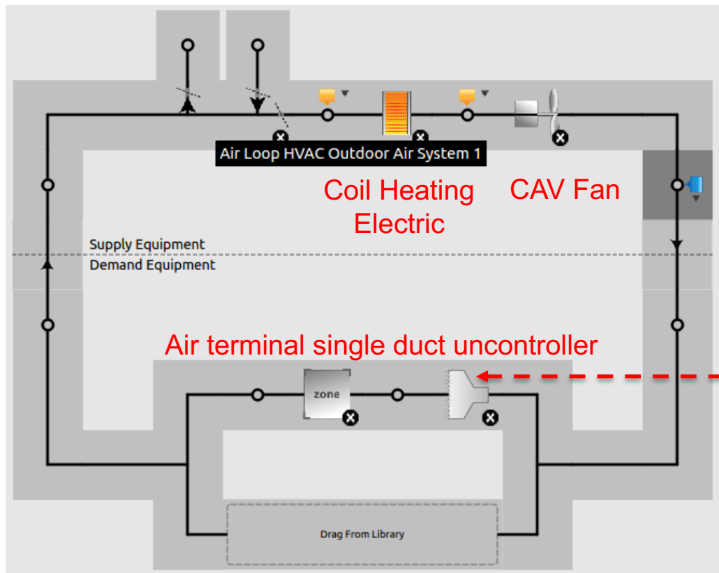
Air Loop
