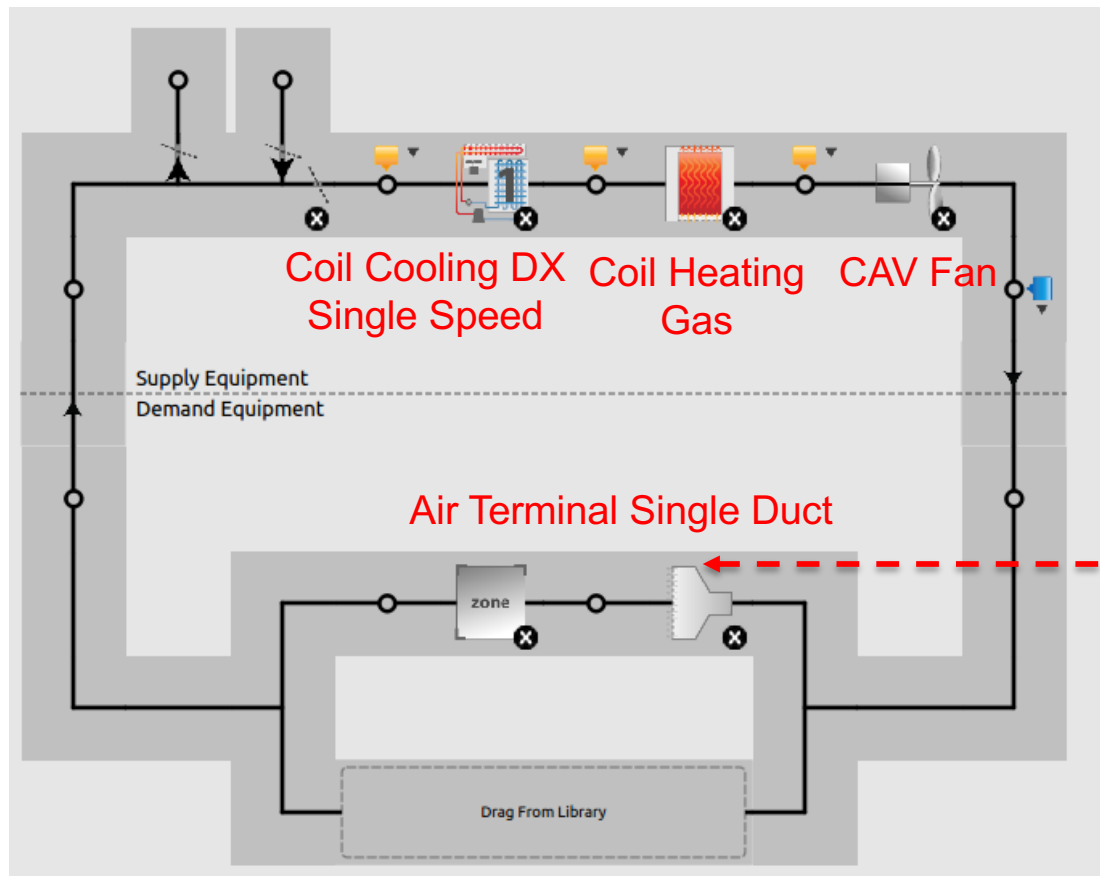
Air Loop
