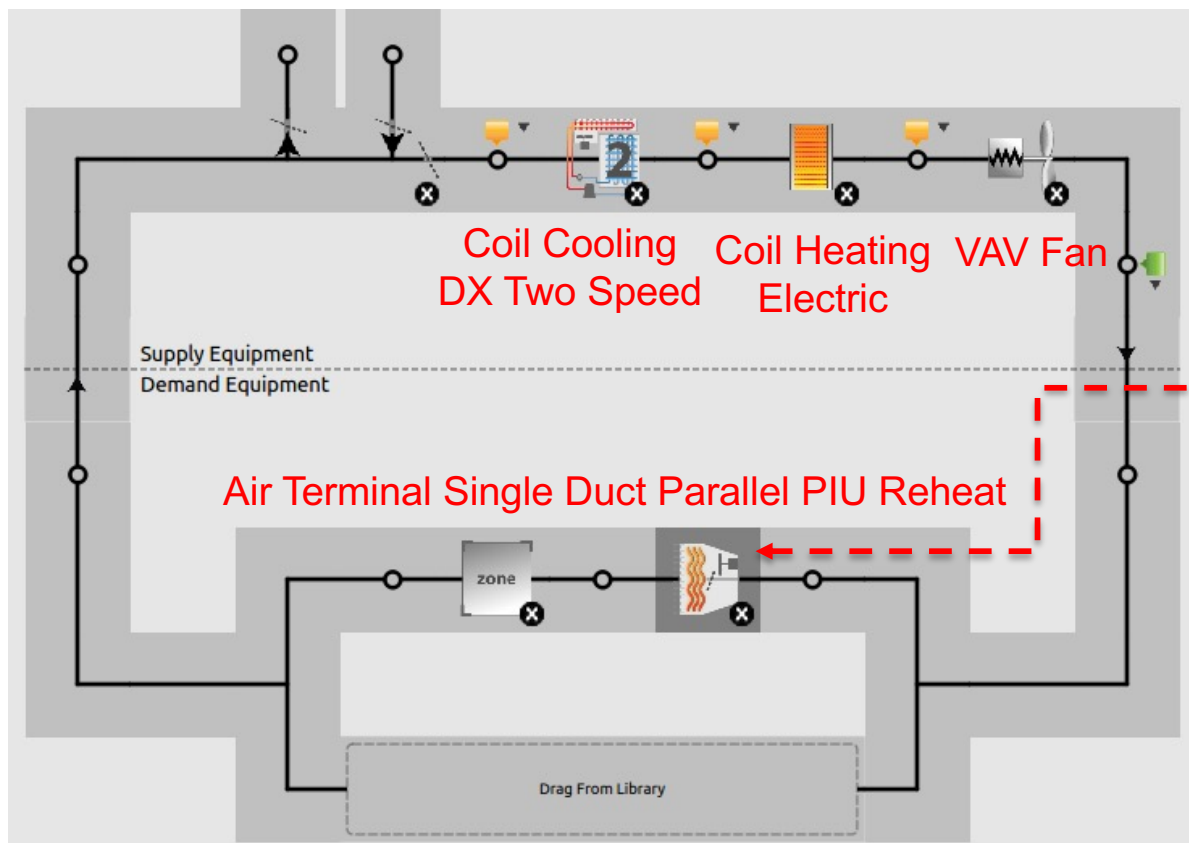
Air Loop
