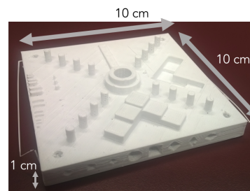
Figure 1. Printed standardized test part from NIST used for emissions testing
