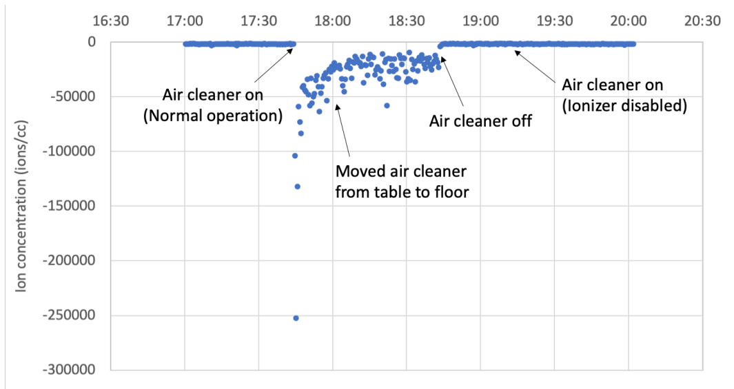
Figure 3. Time-series ion concentrations measured in the chamber during normal operation (no pollutant injection) with the ionizer enabled (default) and then with the ionizer disabled
