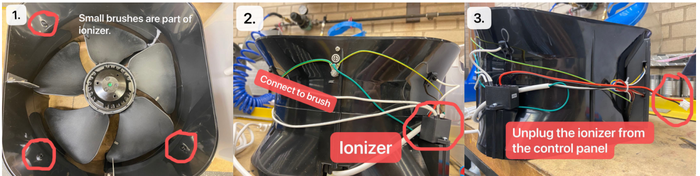
Figure 1. Steps taken to disable ionizer on the unit
