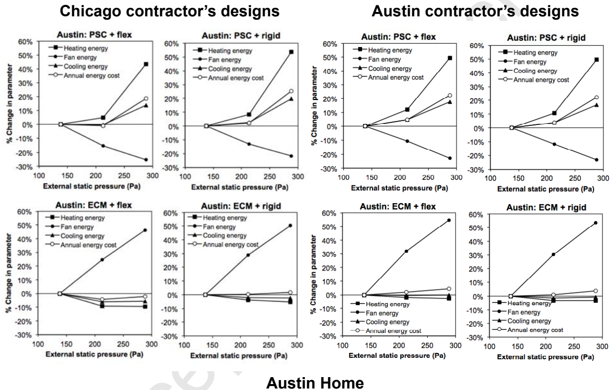
Figure 3. Estimated relative change in annual fan, cooling, and heating energy usage and total annual combined heating and cooling energy costs for the Austin home with both types of AHU blowers and both rigid and flex duct work at each duct design from both contractors.
