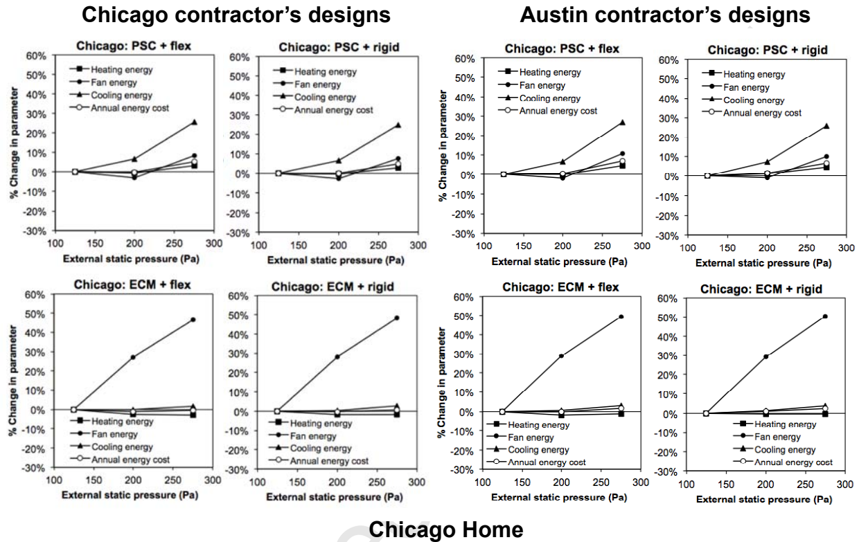
Figure 2. Estimated relative change in annual fan, cooling, and heating energy usage and total annual combined heating and cooling energy costs for the Chicago home with both types of AHU blowers and both rigid and flex duct work at each duct design from both contractors.
