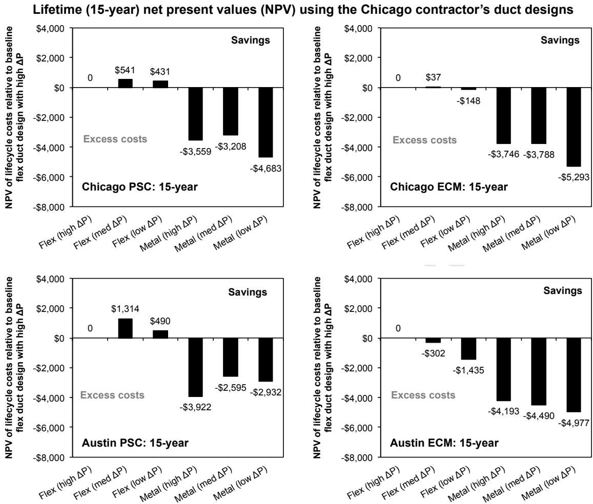
Figure 6. Net present value (NPV) of the life cycle costs of both flex and rigid duct designs over 15-year life relative to the high pressure flex duct condition in each location and with each type of blower installed. Duct designs are limited only to the Chicago contractor's for clarity. The high pressure case refers to 275 Pa of total pressure for the Chicago home and 288 Pa of total pressure for the Austin home. Positive values represent scenarios with life cycle cost savings.
