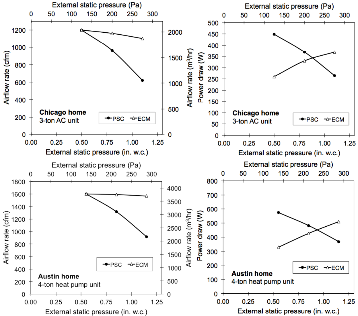
Figure 1. Fan airflow rate and power draw inputs utilized at each of the low, medium, and high external static pressures in this work for both PSC and ECM blowers.
