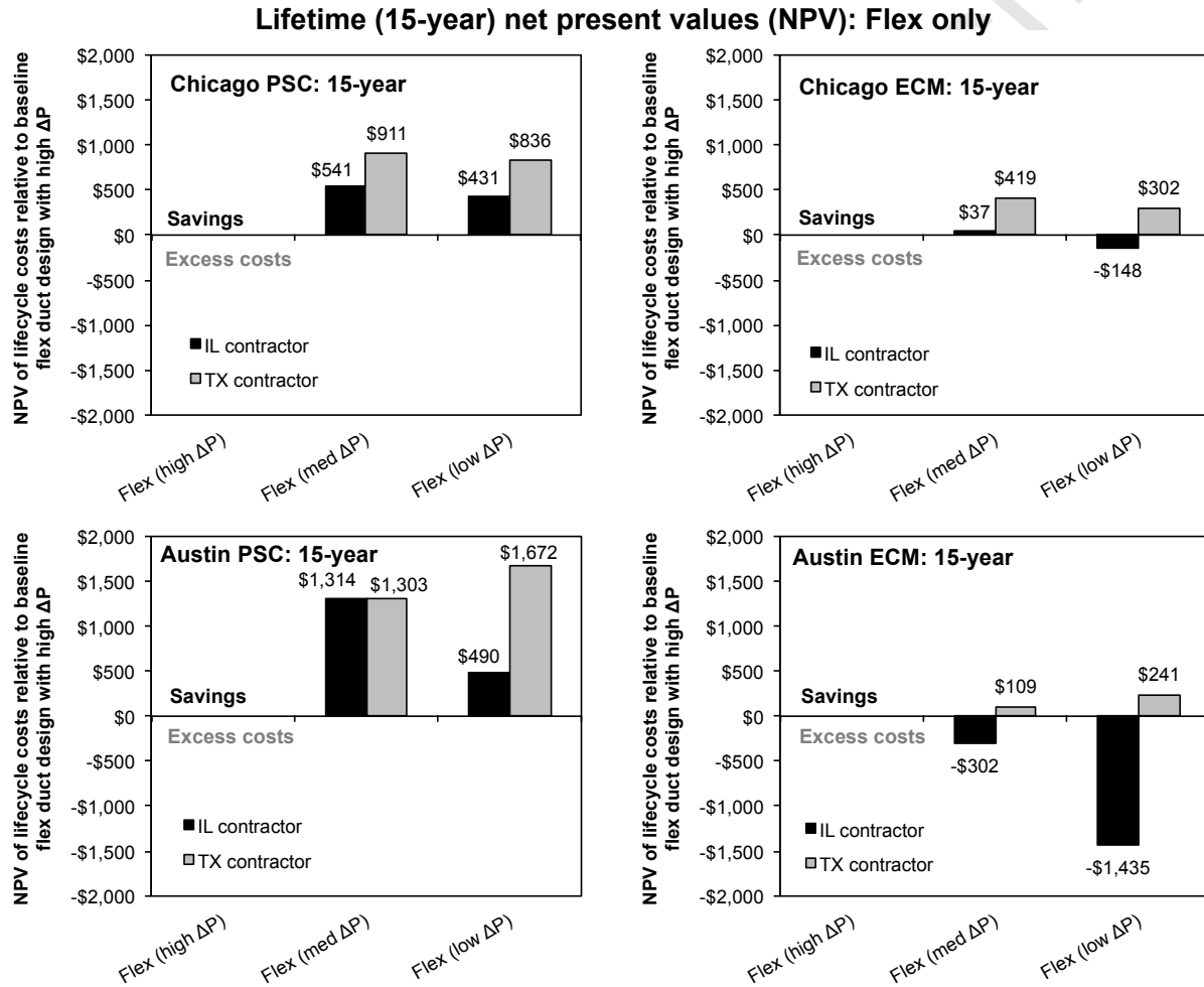
Figure 4. Net present value (NPV) of the life cycle costs of flex duct designs over 15-year life relative to a high pressure flex duct design in each location and with each type of blower installed and duct designs from both contractors. The high pressure case refers to 275 Pa of total pressure for the Chicago home and 288 Pa of total pressure for the Austin home. Positive values represent scenarios with lifetime savings.
