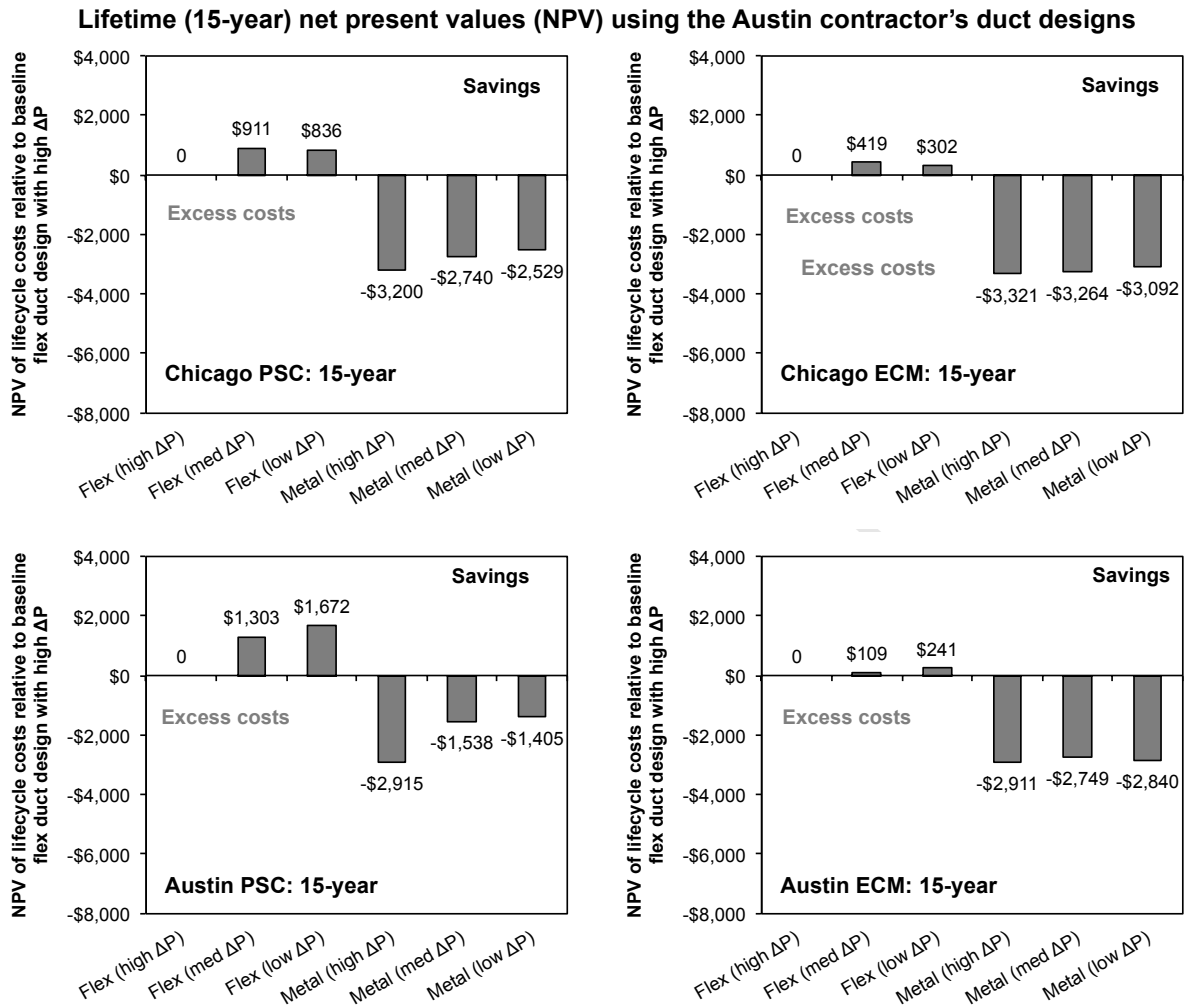
Figure 7. Net present value (NPV) of the life cycle costs of both flex and rigid duct designs over 15-year life relative to the high pressure flex duct condition in each location and with each type of blower installed. Duct designs are limited only to the Austin contractor's for clarity. The high pressure case refers to 275 Pa of total pressure for the Chicago home and 288 Pa of total pressure for the Austin home. Positive values represent scenarios with life cycle cost savings.
