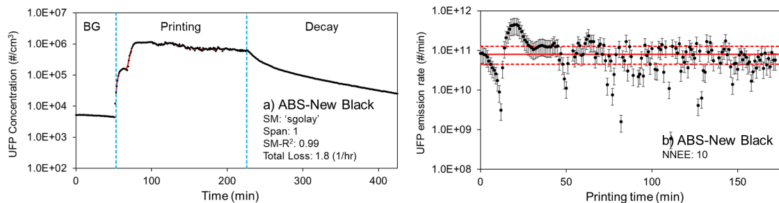
Figure 2. a) Time-varying UFP concentrations inside the chamber during background, printing, and decay time periods, and b) estimates of time-varying UFP emission rates during the printing period
