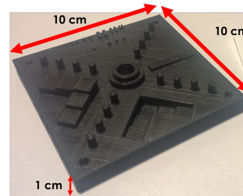
Figure 1. Printed standardized test part from NIST used for emissions testing
