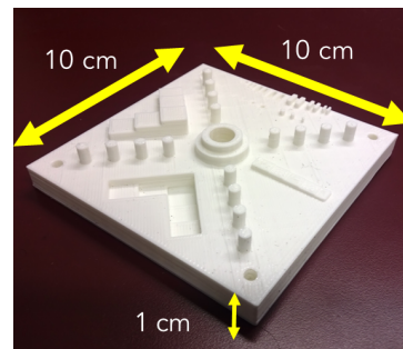
Figure 1. Printed standardized test part from NIST used for emissions testing
