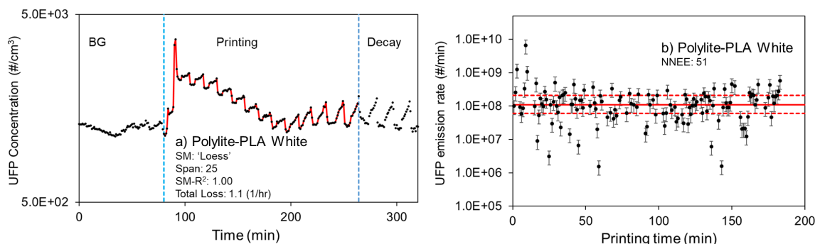
Figure 2. a) Time-varying UFP concentrations inside the chamber during background, printing, and decay time periods, and b) estimates of time-varying UFP emission rates during the printing period
